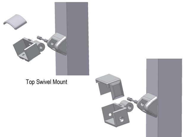
Bottom and Mid Swivel Mount
